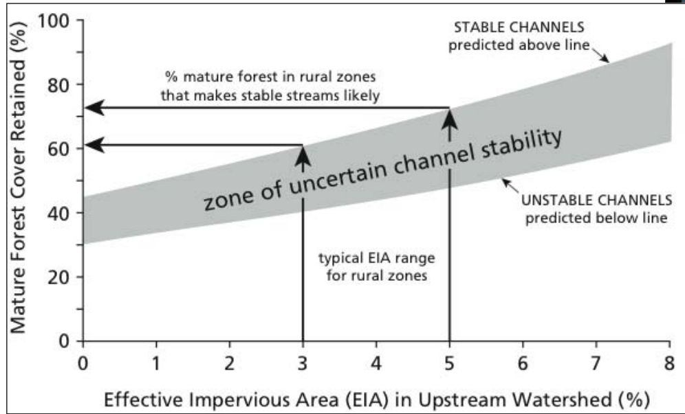
Figure C4.12. Predicted stream channel stability in relation to forest cover and effective impervious area (hydraulically connected to the stream) (de la Crétaz and Barten, 2007: 290 adapted from Booth et al., 2002).
