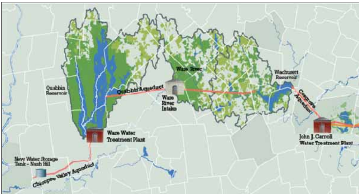
Figure C4.9. Quabbin, Reservoir, Ware River, and Wachusett Reservoir water supply serving 2.2 million consumers in the Boston Metropolitan Area and Chicopee Valley (Kyker-Snowman, 2010).
