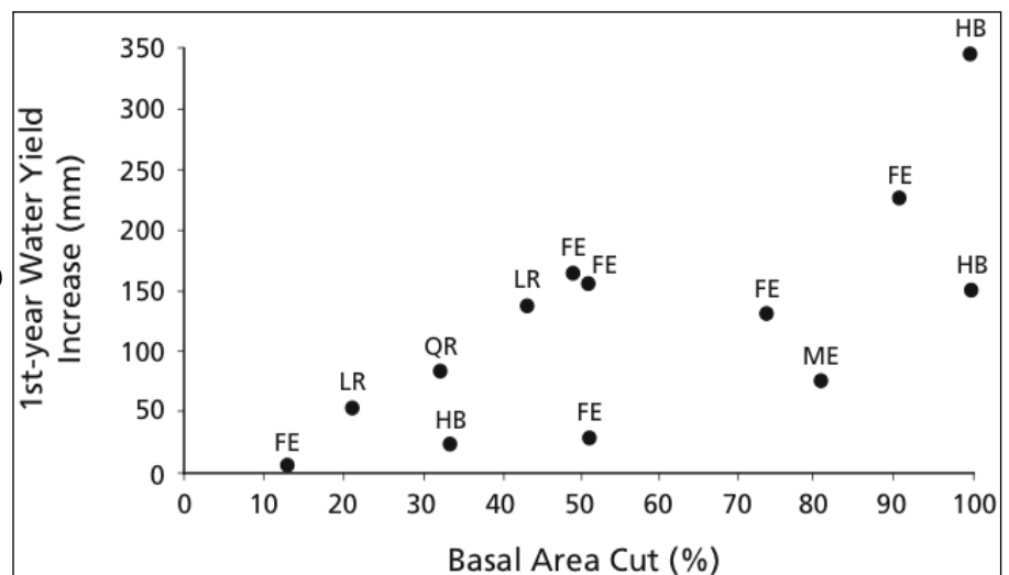
Figure C4.1. First-year water yield increases versus cutting: FE, Fernow Experimental Forest, West Virginia; LR, Leading Ridge Experimental Forest, Pennsylvania; QR, Quabbin Reservoir, Massachusetts; ME, Marcell Experimental Forest, Minnesota (de la Cr  taz and Barten, 2007).
