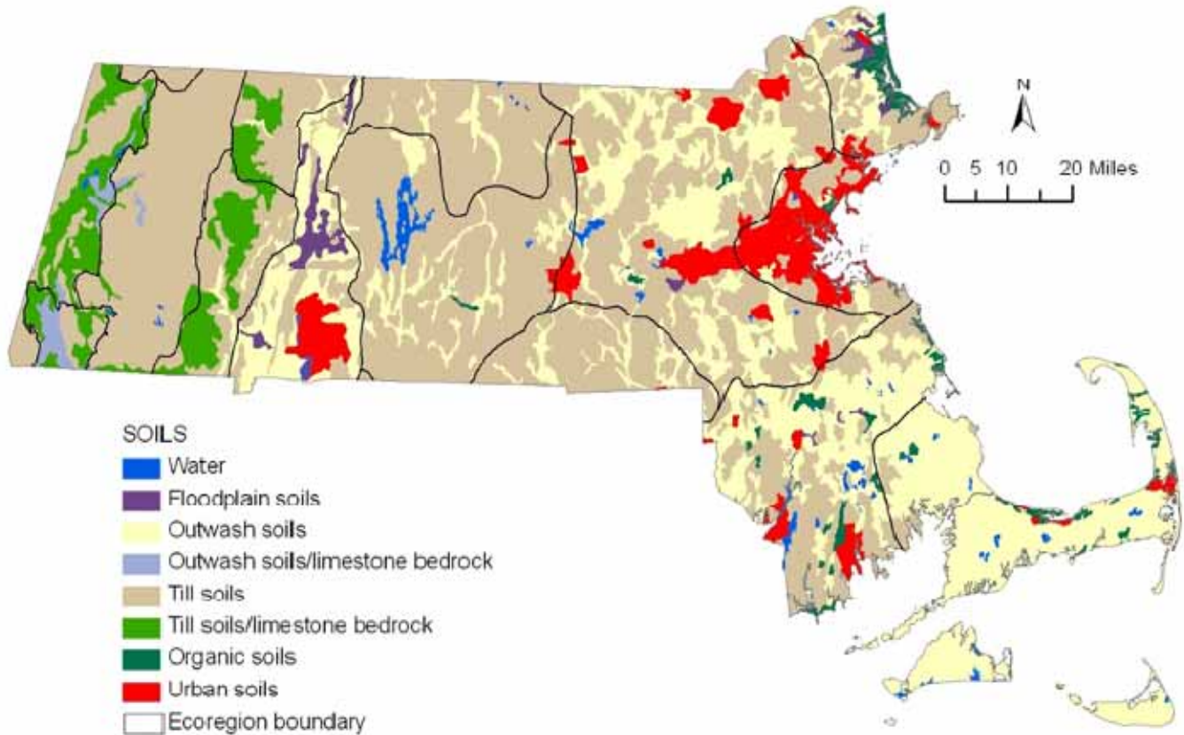
Figure C4.2. Soils grouped by glacial origin (Soil Survey Staff, NRCS, 2006).
